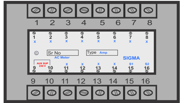
Rear View
